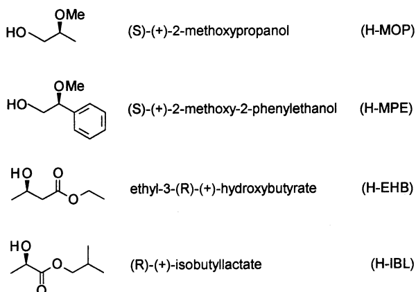
Scheme 1. Formulae, names and abbreviations of the four functionalized alcohols used as ligand precursors.
