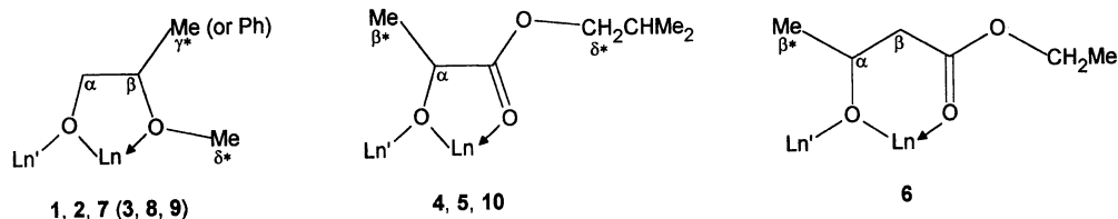
Scheme 2. Survey of the composition of the five- and six-membered rings resulting from intramolecular chelation.
