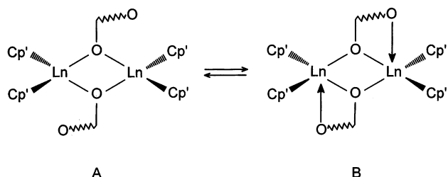
Fig. 1. Schematic view of the two structural alternatives A and B to be expected for all title complexes.
