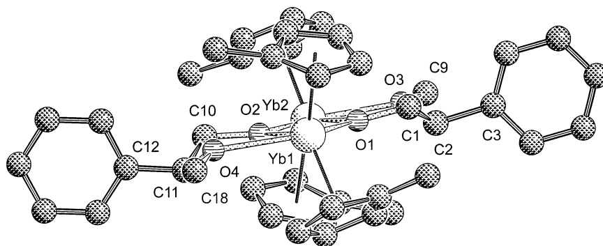
Fig. 4. Alternative perspective (parallel to the Yb 2 O 2 plane) of the structure of 9 (SCHAKAL plot).
