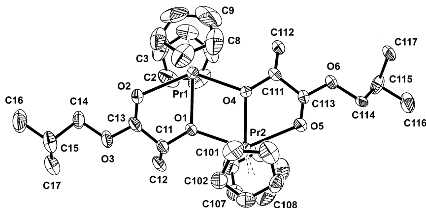
Fig. 2. ORTEP plot with atomic numbering scheme of complex 4.
