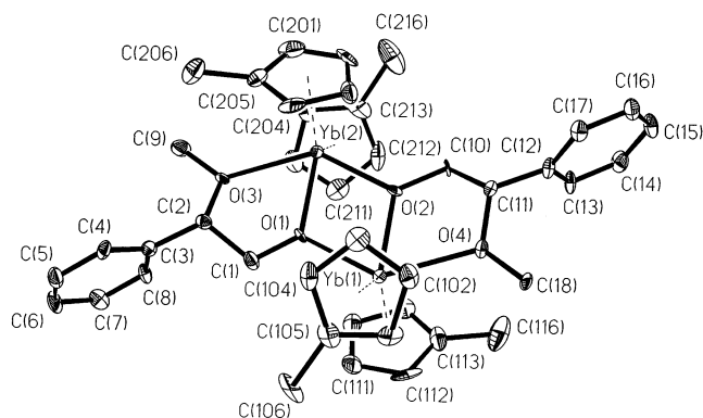
Fig. 3. ORTEP plot with atomic numbering scheme of complex 9 (view upon the \text{Yb}_2\text{O}_2 plane).
