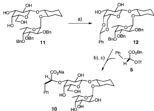
Scheme 2. Synthetic strategy for the target molecules. a) 3.0 equiv \text{PhCH(OMe)}_2 , 0.5 equiv camphorsulfonic acid, MeCN, 35 °C, 0.75 h (87%); b) 1.5 equiv \text{Bu}_2\text{SnO} , MeOH, reflux, 2 h; evaporated; 5 equiv anhydrous CsF, 5 equiv benzyl ( R )-2-phenyl-1-trifluoromethanesulfonyloxypropionate ( 5 ), 1,2-dimethoxyethane, RT, 2 h (70%); c) 20% \text{Pd(OH)}_2/\text{C} , \text{H}_2 , dioxane/ \text{H}_2\text{O}/\text{HOAc} , RT, 1 bar, 7 h, Dowex 50 ( \text{Na}^+ ) (78%).
