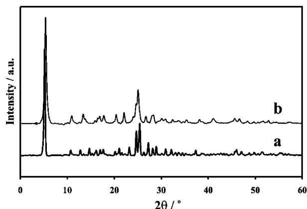
Figure 1. Powder X-ray diffraction patterns of [M_2(pzc)_2(H_2O)_5][Mo_5O_{16}] for I (a, M = Ni ) and II (b, M = Co ).
