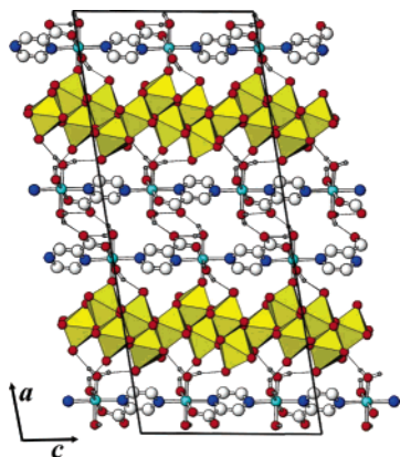
Figure 2. \sim[010] view of the [Ni_2(pzc)_2(H_2O)_5][Mo_5O_{16}] layered structure with the unit cell outlined. Red atoms = O, light blue = Ni, dark blue = N, white = C, and yellow polyhedra = MoO_6 .
