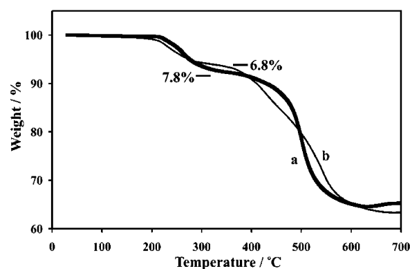
Figure 6. The thermogravimetric analysis of I (a) and II (b) plotted as wt % versus temperature.
