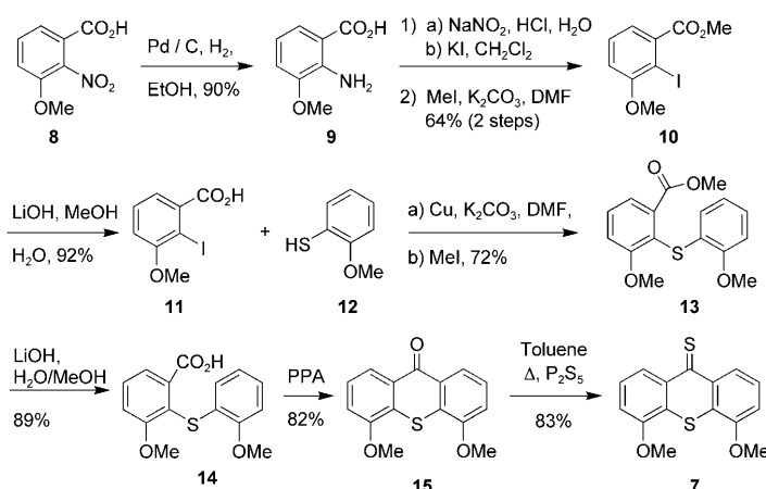
Scheme 2. Initial synthesis of the thioxanthone lower half with two methoxyl groups amenable to further functionalisation.
