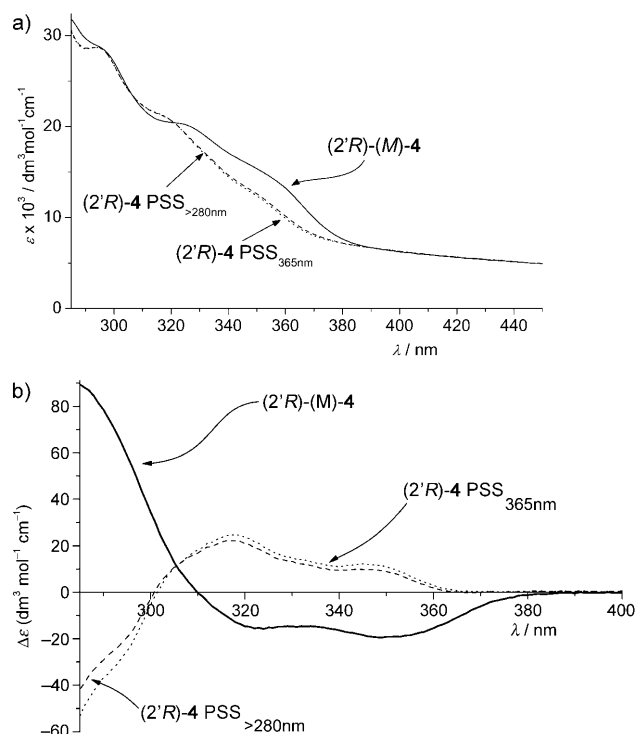
Figure 7. a) UV/Vis spectra of (2'R)-(M)-4 (solid), PSS >280 nm (dashed) and PSS 365 nm (dotted) containing predominantly (2'R)-(P)-4 in toluene. All spectra are adjusted for molar concentration of chromophores. b) CD spectra of pure (2'R)-(M)-4 (solid), PSS >280 nm (dashed), and PSS 365 nm (dotted) in toluene; all spectra are adjusted for molar concentration of chromophores for comparison with (2'R)-(M)-5.
