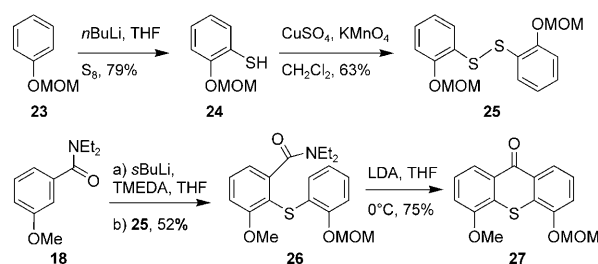
Scheme 5. Synthesis of dissymmetric thioxanthone lower half 27 .
