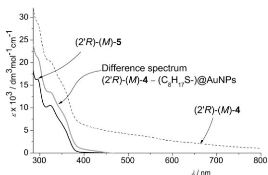
Figure 3. UV/Vis spectra of (2' R )-(M)- 5 (black, solid), (2' R )-(M)- 4 (black, dashed) and the difference spectrum of (2' R )-(M)- 4 versus the UV/Vis spectrum of gold nanoparticles protected with octanethiol (grey).
