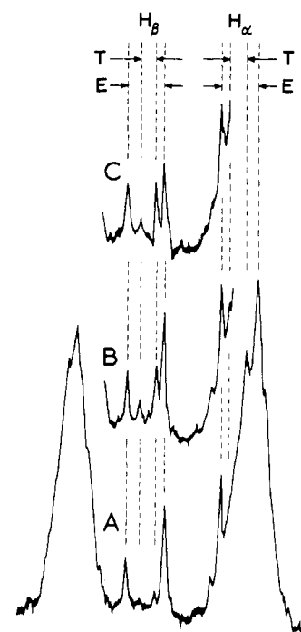
Figure 2. 2 H-Decoupled 1 H NMR spectra of: (A) 2i containing traces of 2k ; (B) organometallic product of reaction of 2i (as in A above) (2.5 × 10 -3 M) with 4 (2.5 × 10 -3 M) after 5400 s at 28 °C in methanol; (C) the organometallic product of reaction of 2i (5 × 10 -3 M) with 6 (5 × 10 -3 M) after 6900 s at 28 °C in methanol. E and T indicate the positions of resonances of the erythro and threo complexes 2i and 2k respectively.
