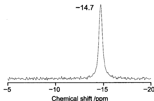
Figure 2. ^{31}\text{P} NMR spectrum of (\text{NH}_4)_3\text{PW}_{12}\text{O}_{40} single crystals.
