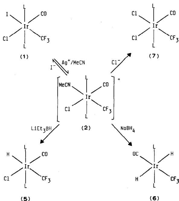
SCHEME 2. L = PPh 3 .
