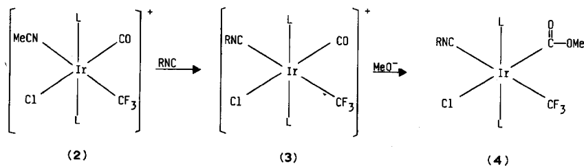
SCHEME 1. L = \text{PPh}_3 , R = p -tolyl.
