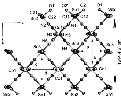
Fig. 1. View on the fragment of one [(\text{Me}_2\text{Sn})\{\text{Me}_2\text{Sn}(\text{H}_2\text{O})_2\}_2\text{-}\{\text{Co}(\text{CN})_6\}_2] ribbon of 1 (extending along c ), including the atomic numbering scheme. Hydrogen atoms have been omitted. a = \text{Sn}3 \cdots \text{Sn}3' : 763.3(3) pm, b = \text{Co}1 \cdots \text{Co}1' : 742.8(3) pm; c = \text{Sn}1 \cdots \text{Sn}3 : 757.0(3) pm, d = \text{Co}1 \cdots \text{Co}1' : 745.0(3) pm.
