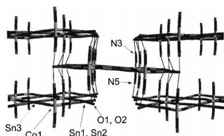
Fig. 2. Supramolecular architecture of 1 : view along c , depicting in the a/b plane the traces of five equivalent ribbons. Inter-ribbon \text{O}-\text{H} \cdots \text{NC} hydrogen bonds (see the text) are indicated by faint straight lines. Methyl groups (bonded to Sn atoms) have been omitted.
