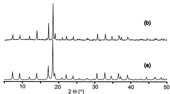
Fig. 3. XRDs of 1 : (a) simulated, (b) experimental diffractogram.
