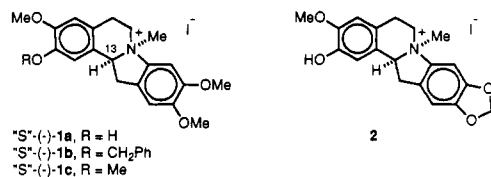
Figure 1. Proposed structures 11,12 for dibenzopyrrocolines 1 and 2.
