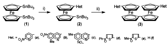
Scheme 2. (i) Het-Br 150% of 1 and 0.5% of \text{PdCl}_2(\text{PPh}_3)_2 in DMF at 100–200 °C heated for 1–1.5 h. (ii) 2 and stoichiometrical \text{CuSO}_4 \cdot 3\text{H}_2\text{O} in THF stirred at r.t. for 1–8 h.
