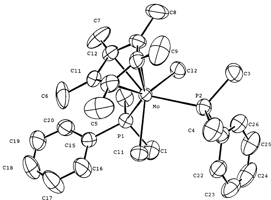
Fig. 2. An ORTEP view of the \text{Cp}^*\text{MoCl}_2(\text{PMe}_2\text{Ph})_2 molecule with the atomic numbering scheme employed. Only the major orientation of the \text{Cp}^* ring is shown. Hydrogen atoms are omitted for clarity.
