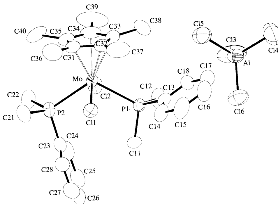
Fig. 3. An ORTEP view of the [\text{Cp}^*\text{MoCl}_2(\text{PMe}_2\text{Ph})_2]\text{AlCl}_4 molecule with the atomic numbering scheme employed. The two fragments are shown in their correct relative orientation. Hydrogen atoms are omitted for clarity.
