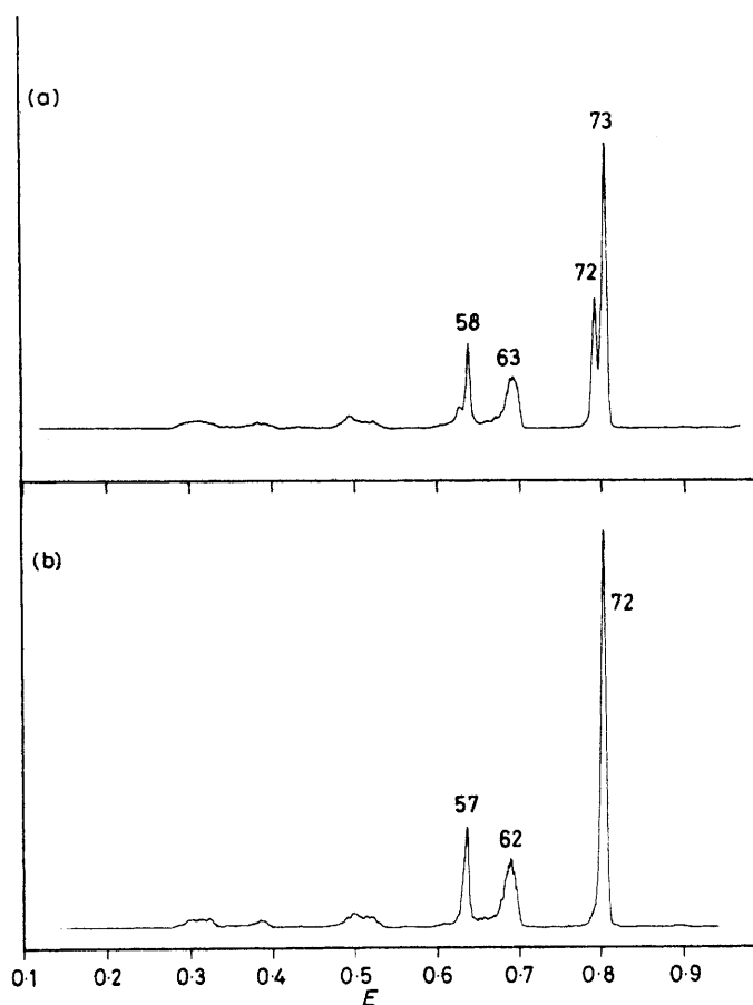
Figure 4. Collision activation mass spectra of the EI-induced molecular ions of the 3-mercaptopropanal (1) ( M^{+\bullet} ) (b) and 3- [^2\text{H}] mercaptopropanal ( M^{+\bullet} ) (a)
