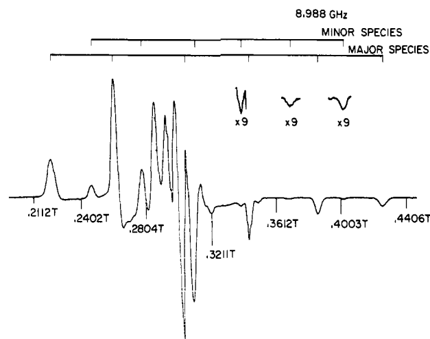
Figure 1. EPR spectrum of a frozen benzene solution (77 K) of \text{Re}(\text{CO})_3(\text{P-c-Hx}_3)_2^{\cdot} . Parallel-field transitions for both major and minor species are indicated.
