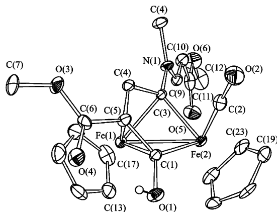
Figure 3. ORTEP drawing of [\text{Fe}_2\{\mu\text{-}\eta^1\text{:}\eta^3\text{-C(OH)C(CO}_2\text{Me)C(H)CN(Me)(CH=CHCO}_2\text{Me)\{CO(Cp)}_2\}}] ( 4 ). Only the hydrogen atom bound to O(1) is shown. Thermal ellipsoids are given at the 30% probability level.
