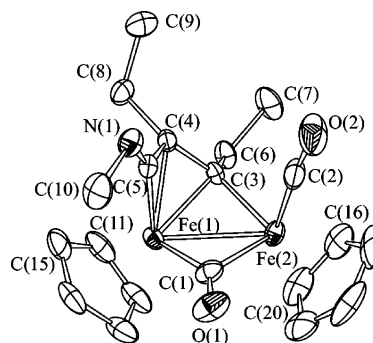
Figure 1. ORTEP drawing of cis - [Fe_2\{\mu-\eta^1:\eta^3-C(Et)C(Et)C=N(Me)\}(\mu-CO)(CO)(Cp)_2] ( 2c ). Hydrogen atoms are omitted for clarity; thermal ellipsoids are given at the 30% probability level.
