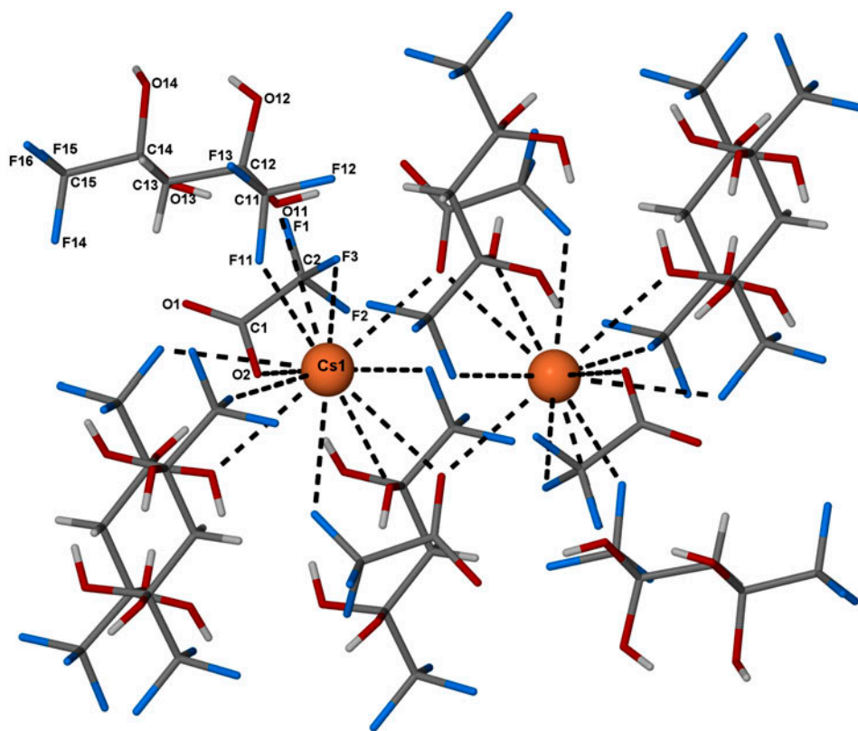
Figure 2. The nearest \text{Cs}^+ environment in the structure of 2 .
