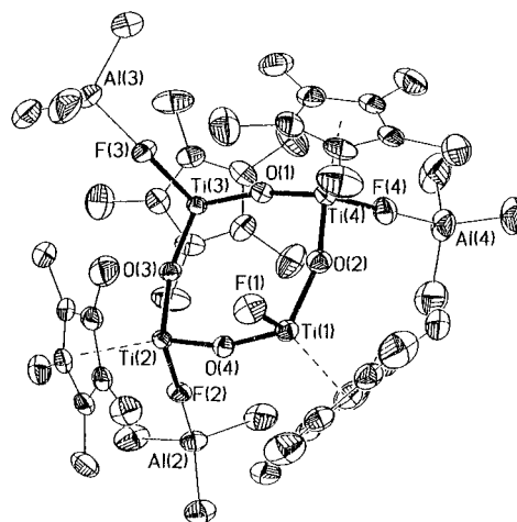
Figure 4. Molecular structure of [\text{C}_5\text{Me}_5\text{Ti}(\mu\text{-O})]_4\text{F}[(\mu\text{-F})\text{AlMe}_3]_3 ( 2b ).
