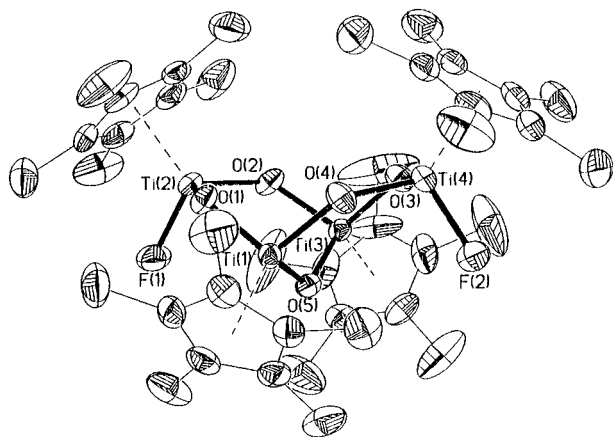
Figure 2. Molecular structure of (\text{C}_5\text{Me}_5)_4\text{Ti}_4\text{O}_5\text{F}_2 ( 1b ).
