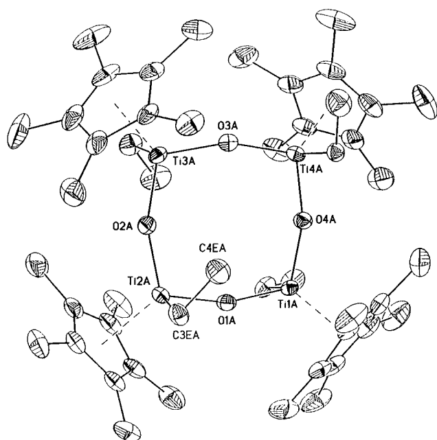
Figure 6. Molecular structure of [\text{C}_5\text{Me}_5\text{Ti}(\mu\text{-O})\text{Et}]_4 ( 4 ).
