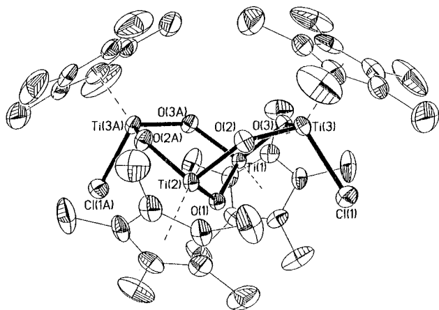
Figure 3. Molecular structure of (\text{C}_5\text{Me}_5)_4\text{Ti}_4\text{O}_5\text{Cl}_2 ( 1a ).
