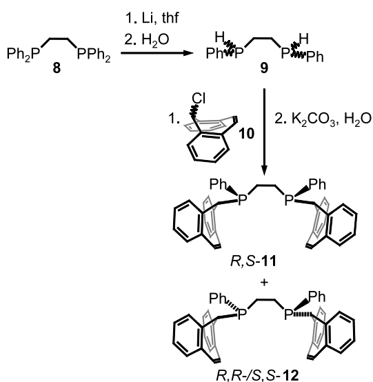
Scheme 2. Synthesis of the bis(tropp) ligands R,S - 11 and R,R -/ S,S - 12 .
