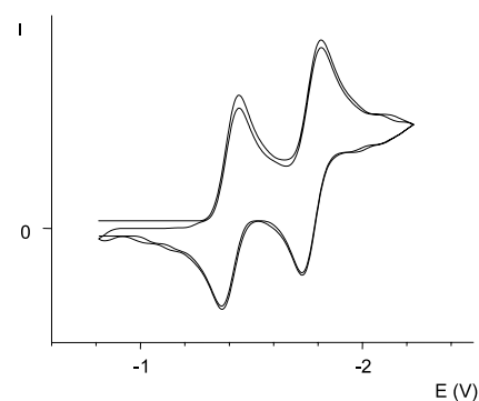
Fig. 3. Cyclic voltammogram of 15 in THF, v = 100 \text{ mV s}^{-1} , T = 20 \text{ °C} .
