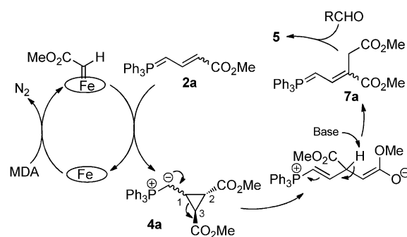
Scheme 3. Proposed mechanism for the diene formation.
