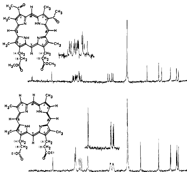
Figure 1. Proton-decoupled natural-abundance carbon-13 Fourier transform nmr spectra at 42° and 15.08 MHz of chloroform solutions of: top, 2,4-diacetyldeuterioporphyrin IX dimethyl ester ( 3 ) (0.15 M and 2886 scans) with the proton decoupling frequency set at about 4 ppm in the proton spectrum (insert, expansion of the region for the nonprotonated carbons of the pyrrole rings); bottom, deuterioporphyrin IX diethyl ester 2 (0.31 M , 530 scans) with the proton decoupling frequency set at about 4 ppm in the proton spectrum (insert, same as the bottom spectrum but with the proton decoupling frequency set at about 1 ppm in the proton spectrum). All spectra were recorded with a 90° pulse recycle time of 5.43 sec. The region shown is from -11.5 to 193.0 ppm from neat carbon disulfide. The intense resonance at 115.4 ppm is from the solvent.
