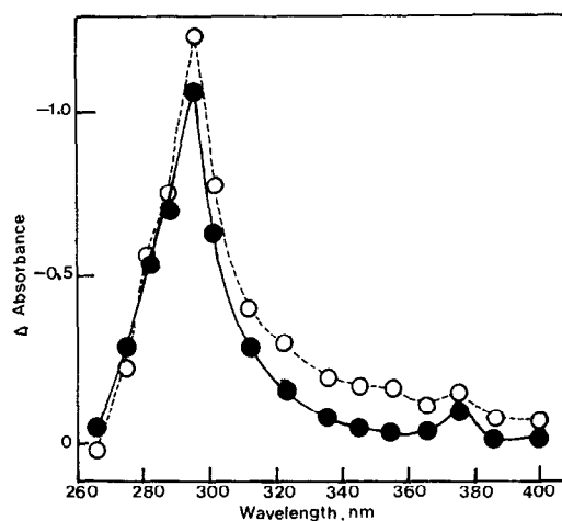
Figure 2. Difference spectra taken after flash photolysis of [\text{W}(\text{N}_2)_2(\text{dppe})_2] in thf saturated with \text{N}_2 . O, immediately following the flash; X, 11.25 msec after the flash at the end of the first stage of the reactions shown in Fig. 1.
