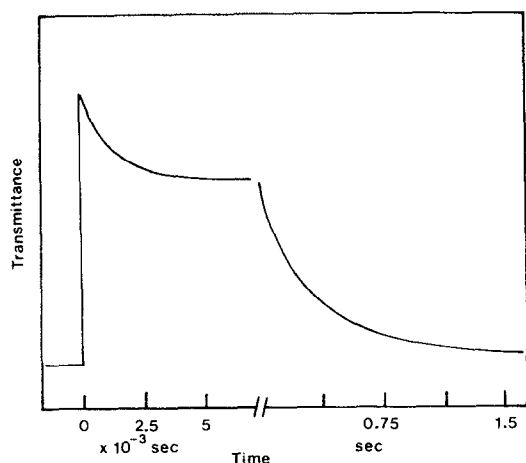
Figure 1. Changes in transmittance at 297 nm following flash photolysis of [\text{W}(\text{N}_2)_2(\text{dppe})_2] , 4 \times 10^{-5} M in thf saturated with \text{N}_2 . Note change of scale on x-axis.
