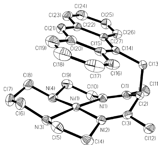
Figure 1. Molecular structure and numbering of atoms for the cation of [Ni(anthracyl diene)]I 2 ( 2b ). Hydrogen atoms are omitted for clarity. Thermal ellipsoids are drawn at the 30% level.
