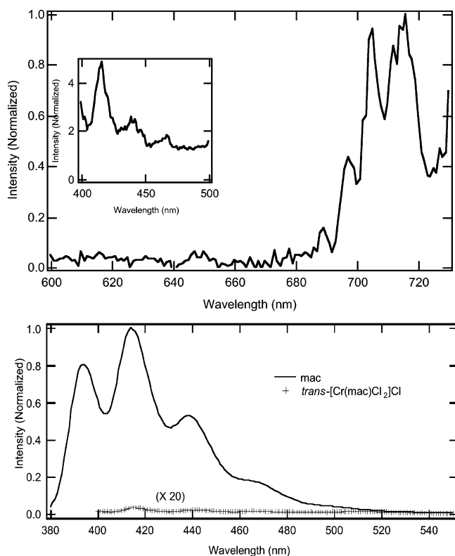
Figure 8. (Top) Emission spectrum for a dilute solution of trans -[Cr(mac)Cl 2 ]Cl ( 5b ) (50 \mu M) in EtOH:MeOH (4:1 v/v) at 77 K ( \lambda_{\text{ex}} = 370 nm) showing both the fluorescence from the aromatic chromophore and phosphorescence from the Cr(III) doublet states. (Bottom) Comparison of emission spectra from free mac (50 \mu M) in aqueous solution vs that from trans -[Cr(mac)Cl 2 ]Cl (50 \mu M) in 4:1 EtOH/MeOH.
