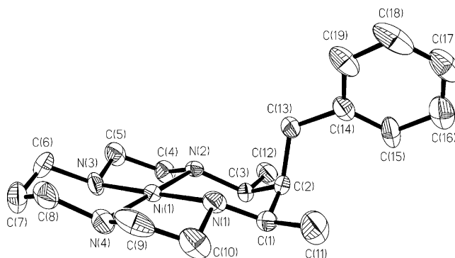
Figure 2. Molecular structure and numbering of atoms for the cation of [Ni(mbc)](ClO 4 ) 2 ( 3a ). Hydrogen atoms are omitted for clarity. Thermal ellipsoids are drawn at the 30% level.
