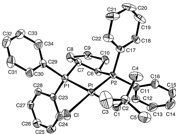
Fig. 3. Molecular structure of [\text{C}_5\text{H}_8(\text{PPh}_2)_2\text{Pt}(\text{Cl})(\text{CH}_2\text{CMe}_3)] , 7 . Selected bond lengths (Å) and valence and torsion angles (°): Pt–Cl, 2.369(1); Pt–P(1), 2.344(1); Pt–P(2), 2.208(1); Pt–C(1), 2.101(5). Cl(1)–Pt(1)–P(1), 91.65(5); Cl(1)–Pt(1)–P(2), 173.52(7); Cl(1)–Pt(1)–C(1), 87.8(1); P(1)–Pt(1)–P(2), 86.74(5); P(1)–Pt(1)–C(1), 175.6(2); P(2)–Pt(1)–C(1), 93.3(1). P(1)–Pt(1)–P(2)–C(11), -140.0(2) ; P(1)–Pt(1)–P(2)–C(17), 90.5(2) ; P(2)–Pt(1)–P(1)–C(23), 110.6(2) ; P(2)–Pt(1)–P(1)–C(29), -124.9(2) .
