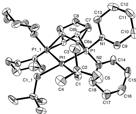
Fig. 6. Molecular structure of [\text{C}_5\text{H}_8\{\text{P}(\text{N-pip})_2\}_2\text{Pt}(\text{CH}_2\text{CMe}_3)_2] ( 10 ) showing the twofold spatial disorder of ring atoms C(6a) and C(6b). Selected bond lengths (Å) and valence and torsion angles (°): Pt(1)–P(1), 2.285(1); Pt(1)–C(1), 2.135(5). P(1)–Pt(1)–P(1)_1, 86.38(7); P(1)–Pt(1)–C(1), 90.4(1); P(1)–Pt(1)–C(1)_1, 176.3(1); C(1)–Pt(1)–C(1)_1, 92.8(3). P(1)_1–Pt(1)–P(1)–N(1), 125.2(2) ; P(1)_1–Pt(1)–P(1)–N(2), -110.9(2) . Operators for generating equivalent atoms P(1)_1 and C(1)_1: -x, y, -z + \frac{1}{2} .
