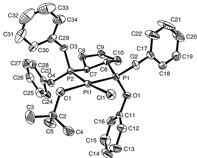
Fig. 5. Molecular structure of [\text{C}_5\text{H}_8\{\text{P}(\text{OPh})_2\}_2\text{Pt}(\text{Cl})(\text{CH}_2\text{CMe}_3)] , 9 . Selected bond lengths (Å) and valence and torsion angles (°): Pt(1)–Cl(1), 2.359(1); Pt(1)–P(1), 2.277(1); Pt(1)–P(2), 2.181(1); Pt(1)–C(1), 2.108(5). Cl(1)–Pt(1)–P(1), 90.99(5); Cl(1)–Pt(1)–P(2), 172.73(5); Cl(1)–Pt(1)–C(1), 88.8(2); P(1)–Pt(1)–P(2), 85.26(5); P(1)–Pt(1)–C(1), 177.9(2); P(2)–Pt(1)–C(1), 95.2(2). P(1)–Pt(1)–P(2)–O(3), -97.5(2) ; P(1)–Pt(1)–P(2)–O(4), 136.4(2) ; P(2)–Pt(1)–P(1)–O(1), -106.0(2) ; P(2)–Pt(1)–P(1)–O(2), 131.3(2) .
