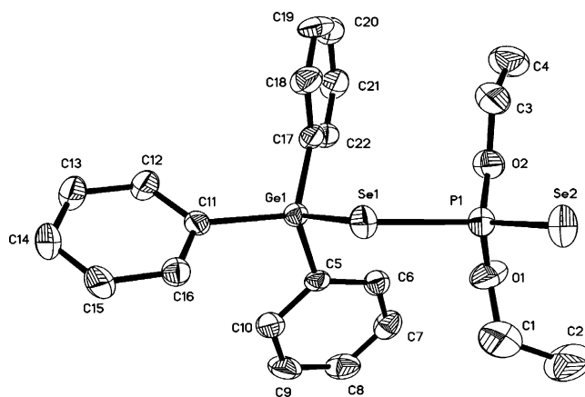
Figure 1. Thermal ellipsoid drawing (30% probability) of [(C 6 H 5 ) 3 Ge{η 1 -Se(Se)P(OEt) 2 }] 2 , 1 , with atomic numbering scheme.
