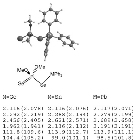
Figure 3. Calculated structural parameters for [\text{Ph}_3\text{M}-(\eta^1\text{-Se}(\text{Se})\text{P}(\text{OMe})_2)] together with those observed (in parentheses) experimentally for 1 , 4 and 7 . The bond distances are given in angstroms and the bond angles are given in degrees.
