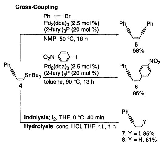
Scheme 6.
