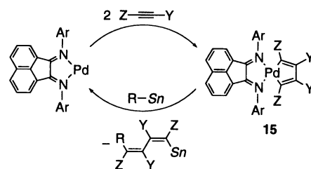
Scheme 11.
