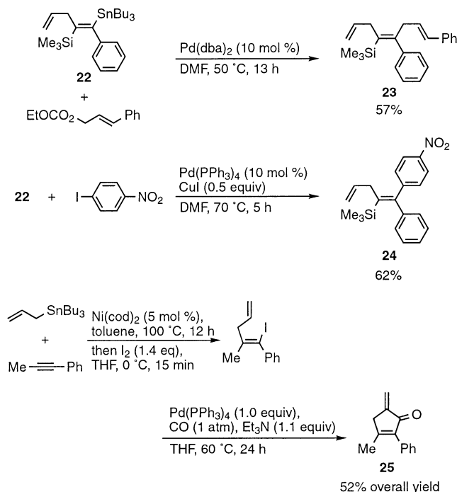
Scheme 15.
