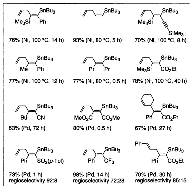
Scheme 13.
