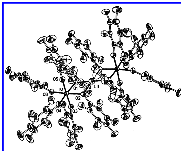
Figure 2. ORTEP plot (50% probabilities on thermal ellipsoids) of polynuclear perfluorophenoxide complexes 5 . \text{M} = \text{Nb} ( 5b ).
