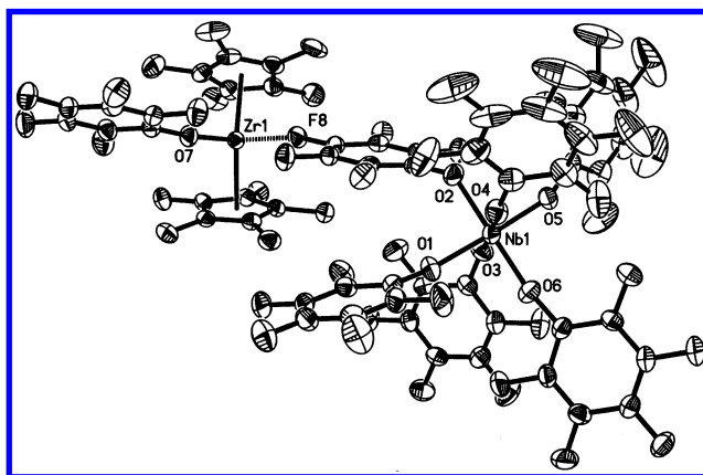
Figure 4. Solid-state structure of [(C_5Me_5)_2Zr(OC_6F_5)]^+ Nb(OC_6F_5)_6^- ( 7 ). Selected bond distances (Å) and angles (deg): Zr1–Cent1 = 2.205(4); Zr1–Cent2 = 2.213(4); Zr1–F8 = 2.342(2); Zr1–O7 = 1.984(2); C10–F8 = 1.383(4); C–F(av) = 1.344(4); Nb–O(av) = 1.946(3); Cent1–Zr1–Cent2 = 1.378(13); F8–Zr1–O7 = 94.28(9); Zr1–O7–C37 = 168.0(3); Zr1–F8–C10 = 167.7(2); O1–Nb1–O5 = 176.44(11); O2–Nb1–O6 = 178.49(11); O3–Nb1–O4 = 174.76(11); smallest cis O–Nb1–O = 86.84(11); largest cis O–Nb1–O = 93.12(11).
