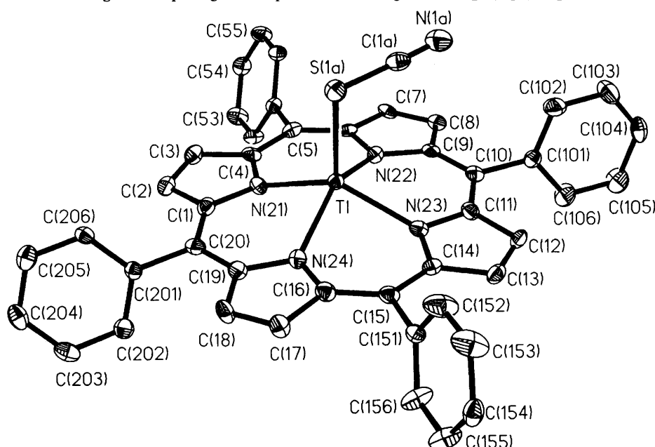
Fig. 7 Computer-generated plot and numbering scheme of [Tl(tpp)(SCN)]
