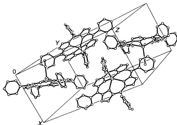
Fig. 10 View of the molecular packing in the unit cell of [\text{Tl}(\text{tpp})(\text{CN})]
