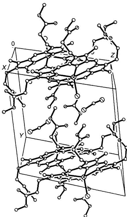
Fig. 9 View of the molecular packing in the unit cell of [\text{TlL}^1(\text{Cl})] . Hydrogen atoms have been omitted for clarity
