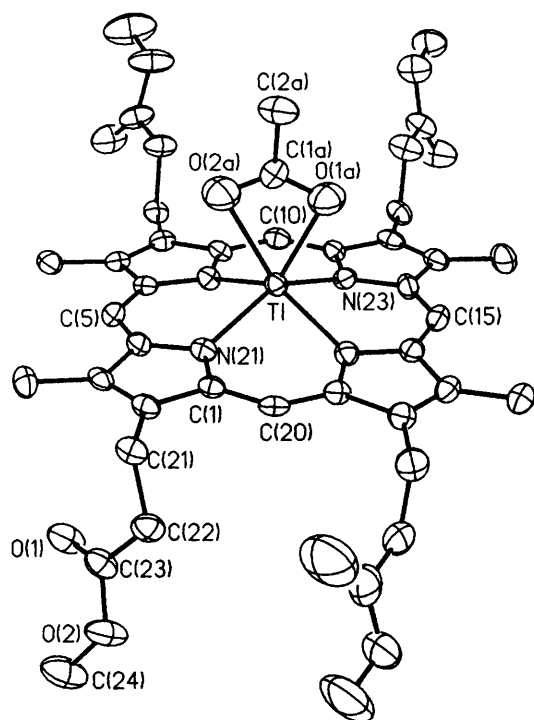
Fig. 1 Computer-generated plot and numbering scheme of [\text{TlL}^2\text{-(O}_2\text{CMe)}] . Hydrogen atoms have been omitted for clarity; ellipsoids at 50% level
