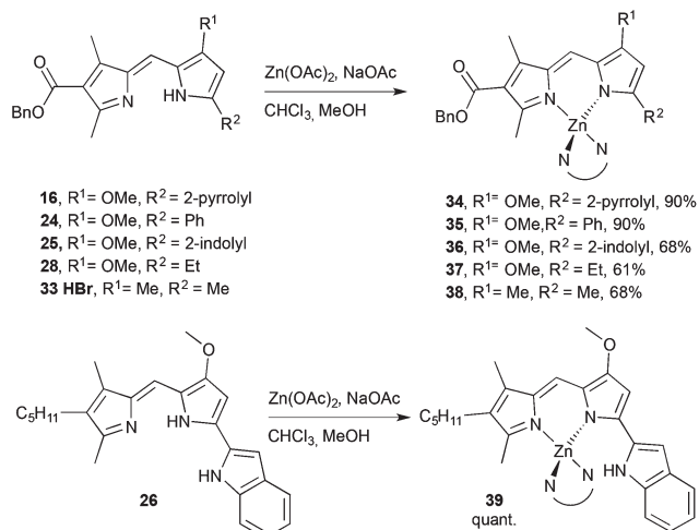
Scheme 6 Synthesis of zinc complexes of prodigiosenes and dipyririns.
