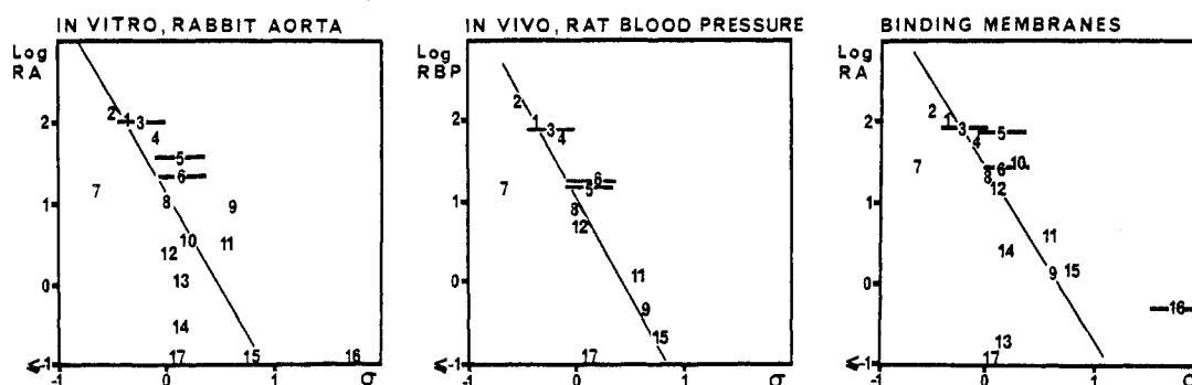
Figure 1. Correlation of electronegativity vs. relative affinity of position-4 modified [Sar 1 ]-angiotensin II analogues on three bioassays. \sigma is the Hammett factor (expression for electronegativity) of the aromatic side chain substituent of position 4 according to Hansch. 16 The horizontal bars indicate the values of protonated and deprotonated forms if both are reasonably present at physiological pH; otherwise, only the predominant form is considered (e.g., 1 is indicated in its protonated form and 9 in the deprotonated form). The oblique line is a calculated linear regression of all values with exclusion of 17. Compounds with affinities equal or lower than 0.1% are indicated on this line. Correlation coefficients are as follows: for rabbit aorta, 0.7527 ( n = 16 ); for rat blood pressure, 0.8644 ( n = 12 ); for the binding assay, 0.7352 ( n = 16 ); significance in all three is therefore better than 0.001 (highly significant). Numerical values (log RA and \sigma ) are from Table I.
