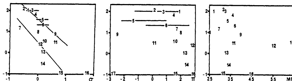
Figure 2. Comparison of physicochemical parameters on position 4 of [Sar 1 ]angiotensin II on rabbit aorta. Left: Correlation between log relative affinity vs. electronegativity ( \sigma ). The upper oblique line represents the linear regression calculated for the Tyr derivatives 1-6 and 9 with an excellent correlation coefficient of 0.9697 (significance better than 0.001). The lower line represents the linear regression calculated for the non-hydroxyl derivatives with a correlation coefficient of 0.7861, n = 9 (significance better than 0.01). Exclusion of 11, which has hydrogen bond acceptor functions, improves the significance to 0.001. The difference between the two regressions is greater than 0.05 (significant). Middle: Correlation between log relative affinity vs. hydrophobicity ( \pi ); correlation coefficient, 0.3715; not significant at 0.1. Right: Correlation between log relative affinity vs. molecular refractivity (MR). No values were available for ionized forms on this plot: correlation coefficient, 0.2906; not significant at 0.1.
