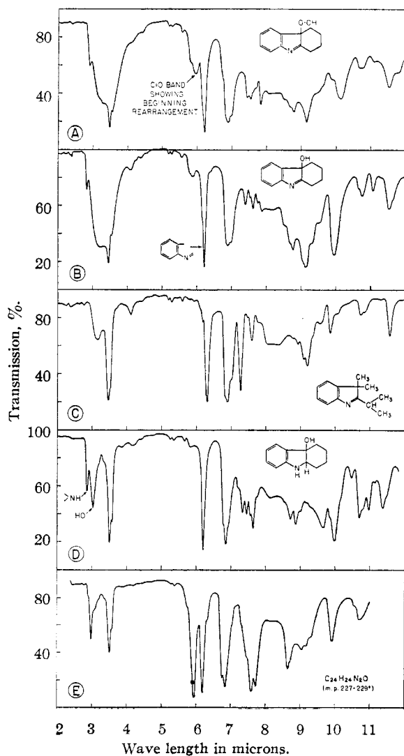
Fig. 1.—Infrared spectra in chloroform.
