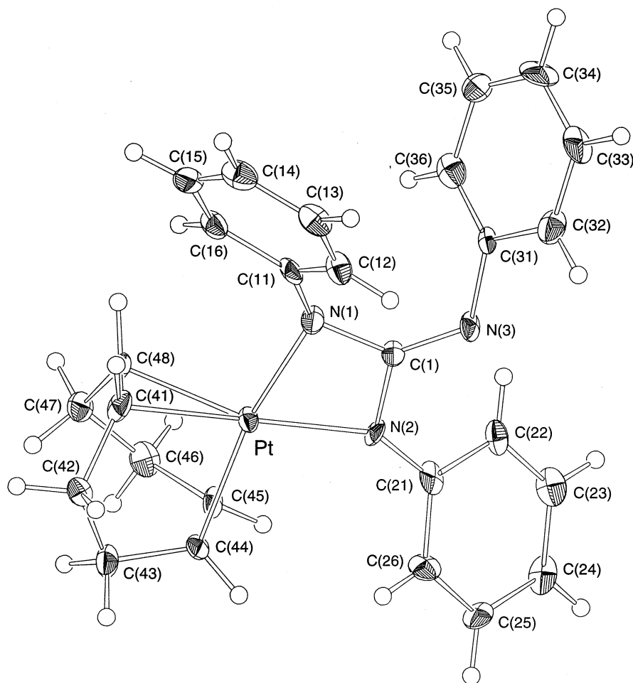
Fig. 1. Molecular structure of [\text{Pt}\{\text{NPhC(=NPh)NPh}\}(\text{COD})] 4a , showing the atom numbering scheme. The dichloromethane and disordered diethyl ether of crystallisation have been omitted for clarity.
