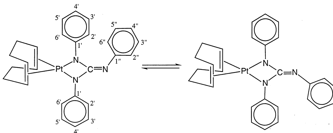
Scheme 2. Fluxional process interconverting the Pt–NR groups, and COD CH and CH 2 groups. The NMR numbering scheme for the phenyl substituents is also shown for the r.t. spectrum with identical Pt–NPh moieties.
