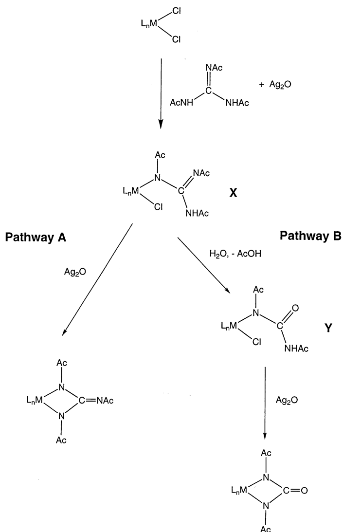
Scheme 1. A possible mechanism explaining the formation of differing amounts of ureylene and guanidine dianion products.
