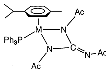
8: M = Ru
