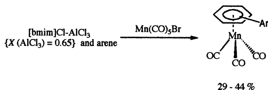
Scheme 3. The synthesis of 6–12 from \text{Mn}(\text{CO})_5\text{Br} {arene = benzene ( 6 ), toluene ( 7 ) mxylylene ( 8 ), mesitylene ( 9 ) biphenyl ( 10 ), [2.2]paracyclophane ( 11 ) or [2.2.2]paracyclophane ( 12 )}.
