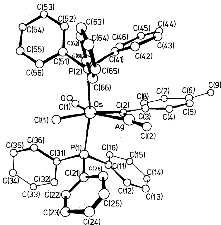
Fig. 2. The molecular geometry and atomic numbering for \text{Os}(\text{C}[\text{AgCl}]\text{R})\text{Cl}(\text{CO})(\text{PPh}_3)_2 ( \text{R} = p\text{-tolyl} ).
