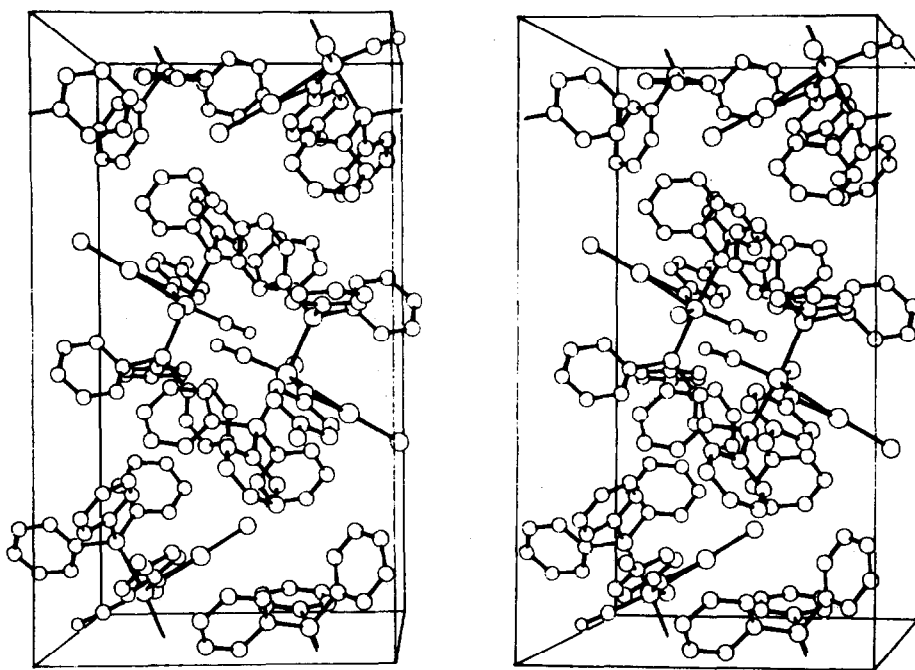
Fig. 3. Stereoview of the molecular packing in \text{Os}(\text{=C}[\text{AgCl}]\text{R})\text{Cl}(\text{CO})(\text{PPh}_3)_2 ( \text{R} = p\text{-tolyl} ).
