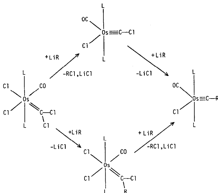
SCHEME 1. Possible mechanisms for the formation of \text{Os}(\equiv\text{CR})\text{Cl}(\text{CO})(\text{PPh}_3)_2 ( \text{R} = p\text{-tolyl} , \text{L} = \text{PPh}_3 ).
