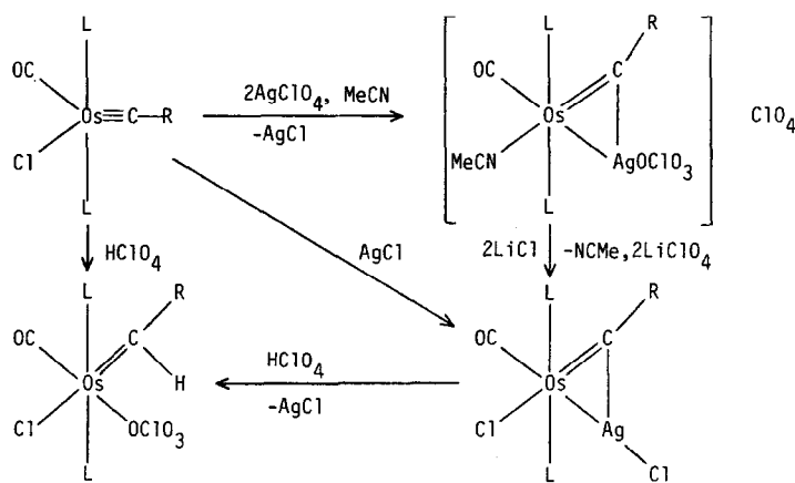
SCHEME 4. Formation of \text{Os}(\equiv\text{C}[\text{AgCl}]\text{R})\text{Cl}(\text{CO})(\text{PPh}_3)_2 ( \text{L} = \text{PPh}_3 , \text{R} = p\text{-tolyl} ).
