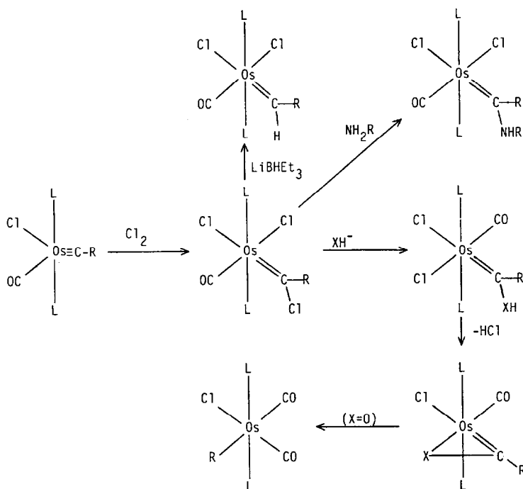
SCHEME 3. Formation and reactions of a chloro- p -tolylcarbene complex ( \text{L} = \text{PPh}_3 , \text{R} = p\text{-tolyl} , \text{X} = \text{O} , S, Se, Te).
