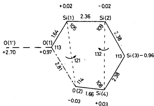
Fig. 2. Geometrical parameters of the pseudocycle in I (distances in Å, angles in °). The deviations of atoms from the mean plane fragment Si(1)Si(2)Si(4)O(2) and the dihedral angles between this plane and the Si(1)O(1)O(2) and Si(2)Si(3)Si(4) moieties are shown. The O(1) and O(1') atoms are linked by the H bond across the symmetry centre.
