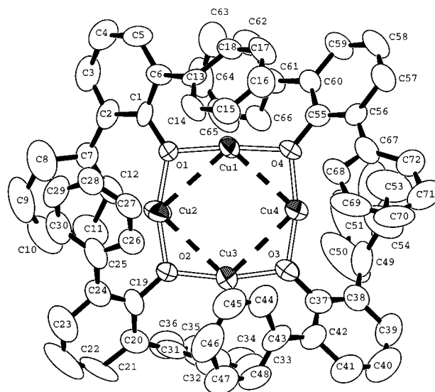
Figure 1. ZORTEP drawing of [(\text{CuOC}_6\text{H}_3\text{Ph}_2)_4] ( 1 ), showing the crystallographic numbering. The \text{Cu}_4\text{O}_4 square in the \text{Cu}_4\text{O}_4 core is emphasized by means of dashed lines.
