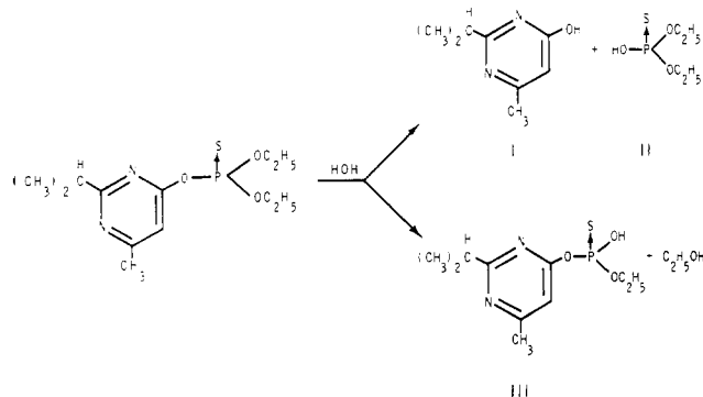
Figure 1. Probable hydrolysis products of Diazinon
