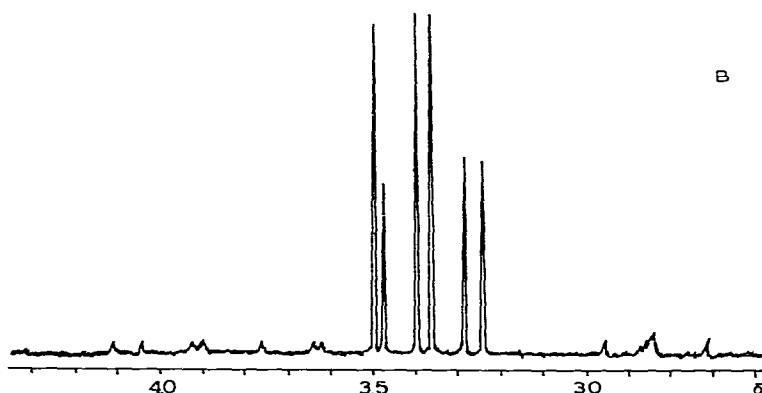
Fig. 3. Part of ^1\text{H} spectrum (180 MHz) of IV, [\alpha]_{\text{D}}^{20} - 5^\circ which represents the methine proton \text{H}-\text{C}-\text{Hg}-\text{C}-\text{H} region; A in \text{C}_5\text{H}_5\text{N} ; V, in \text{C}_6\text{D}_6 .
