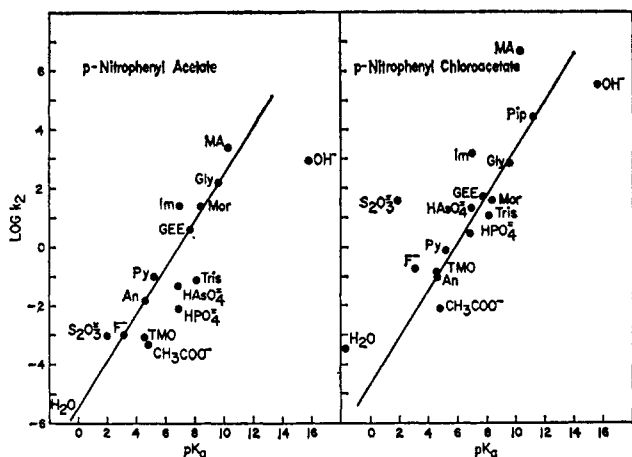
Figure 1. Brønsted plots for reaction of p -nitrophenyl chloroacetate and p -nitrophenyl acetate with a series of nucleophilic reagents in aqueous solution at 25°. Data for the latter plot have been taken from the compilation in ref 15. The abbreviations employed are defined in Table I.
