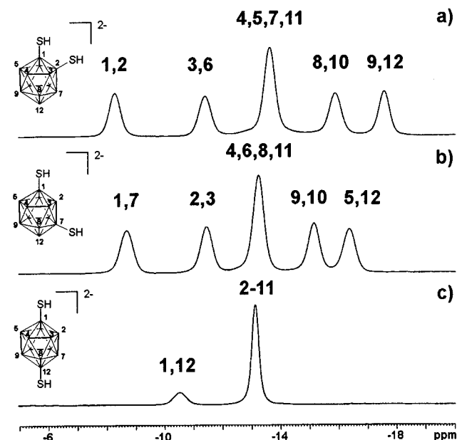
Figure 2. ^{11}\text{B}\{^1\text{H}\} NMR spectra (160.5 MHz) of [1,2-(HS) _2 B _{12} H _{10} ] ^{2-} (7) (a), [1,7-(HS) _2 B _{12} H _{10} ] ^{2-} (8) (b), and [1,12-(HS) _2 B _{12} H _{10} ] ^{2-} (9) (c) in CD _3 CN (cation [n-Bu _4 N] ^+ ).
