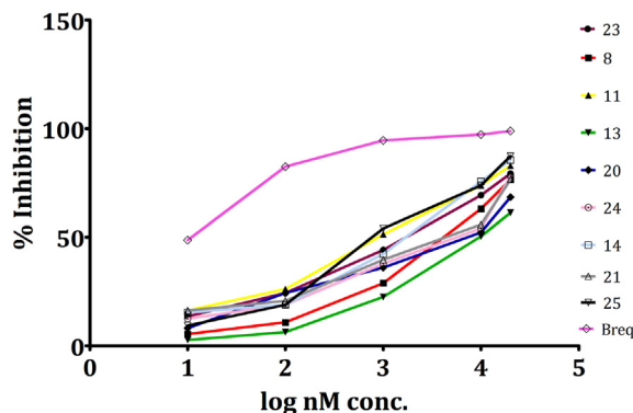
Fig. 3. Dose–response curves for h DHODH inhibition. Five different concentrations 10 nM, 100 nM, 1 \mu M, 10 \mu M and 20 \mu M of the compounds were tasted and IC_{50} values were determined.
