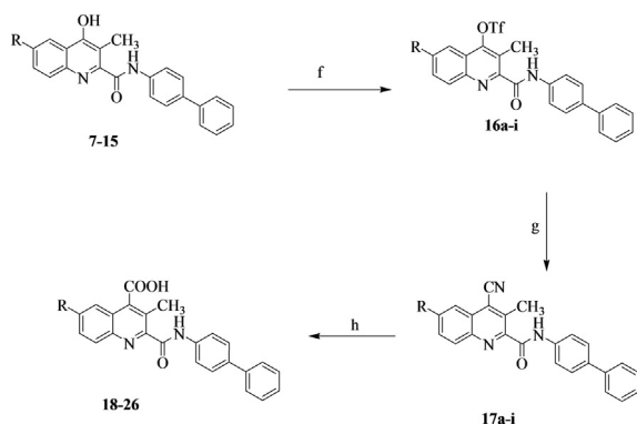
Scheme 3. Synthetic strategy for 6-substituted-4-carboxylic acidquinoline-2-carboxamide derivatives (18–26). (f) TE 2 O, TEA, toluene, stirring 0–5 °C (2 h) to RT 36–42 h, (g) Zn(CN) 2 , Pd(Ph 3 ) 4 , DMF, reflux 20–24 h (h) NaOH, H 2 O.
