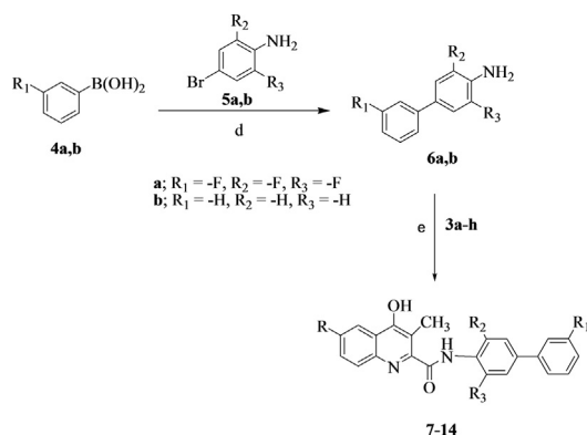
Scheme 2. Synthetic strategy for substituted biphenyl amine derivatives (6a,b) via Suzuki coupling reaction and for 6-substituted-4-hydroxyquinoline-2-carboxamide derivatives (7–14) via acid-amine coupling reaction. Reagents and conditions: (d) Pd(Ph 3 ) 4 , K 2 CO 3 , EtOH, H 2 O, toluene, reflux 14–17 h, (e) TEA, DCC, HOBt, DMF, stirring 0–5 °C (8–12 h) to RT (12–36 h).
