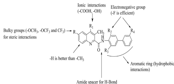
Fig. 2. Design strategy for key structural requirements of quinoline-2-carboxamide derivatives for h DHODH inhibition (hypothetical interaction model).
