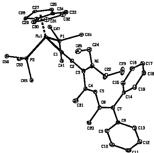
Figure 2. ORTEP view of the molecular structure of the cation of [Ru{C=C=C(NEt 2 )}[(CMe=CH)C(Me)=CPh 2 ]}( \eta^5 -C 9 H 7 )(PPh 3 ) 2 ][PF 6 ] ( 18 ), drawn at the 10% probability level. The hexafluorophosphate anion and phenyl groups of PPh 3 have been omitted for clarity. Only the ipso carbon atoms of the aryl groups are depicted. Selected bond lengths (Å), bond angles (deg), and torsion angles (deg): Ru–P(1) = 2.299(9), Ru–P(2) = 2.305(9), Ru–C(1) = 1.946(4), C(1)–C(2) = 1.229(5), C(2)–C(3) = 1.390(5), C(3)–C(4) = 1.500(5), C(4)–C(5) = 1.340(6), C(5)–C(6) = 1.510(5), C(6)–C(7) = 1.355(5), C(3)–N(1) = 1.319(5); Ru–C(1)–C(2) = 174.6(3), C(1)–C(2)–C(3) = 177.8(4), C(2)–C(3)–N(1) = 122.1(3), C(4)–C(3)–N(1) = 119.0(3), C(2)–C(3)–C(4) = 118.4(2), C(3)–N(1)–C(24) = 121.7(3), C(3)–N(1)–C(22) = 122.1(4), C(24)–N(1)–C(22) = 116.2(4); C(20)–C(6)–C(5)–H(5) = 162.8(3), N(1)–C(3)–C(4)–C(21) = 78.8(5).
