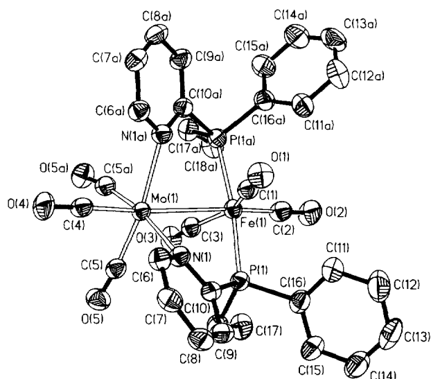
Fig. 1. Perspective view of (CO) 3 Fe(μ-EtPhPpy) 2 Mo(CO) 3 , 2 , in its 2:1 solvate with toluene. The thermal ellipsoids are drawn at the 35% probability level. The atoms Mo(1), Fe(1), C(1), O(1), C(2), O(2), C(3), O(3), C(4) and O(4) lie on a crystallographic mirror plane.
