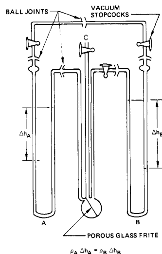
Figure 2. Density cell
