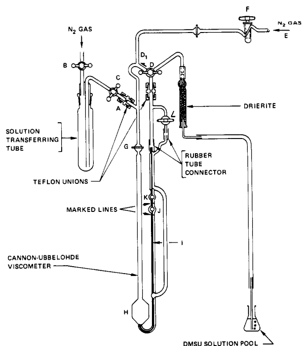
Figure 1. Modified viscometer cell
