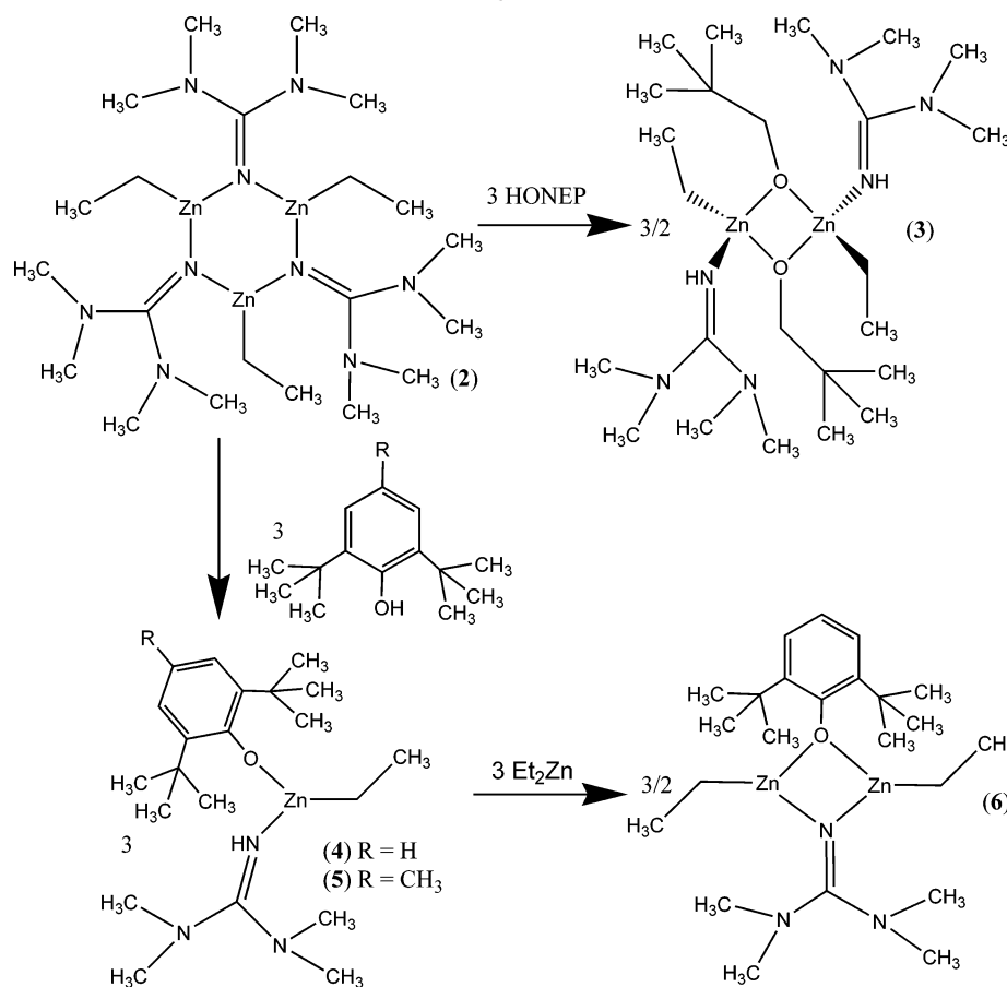
Scheme 3. Synthesis of 7–9
