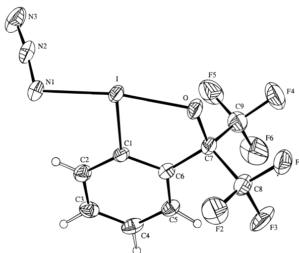
Figure 1. ORTEP representation of the molecular structure of azidobenziodoxole 4b .
