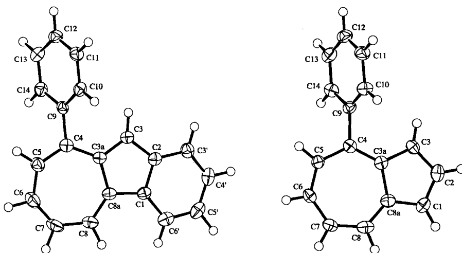
Fig. 2. X-Ray crystal structures of 9-phenylbenz[ a ]azulene ( 4 ) and 4-phenylazulene ( 5 )
