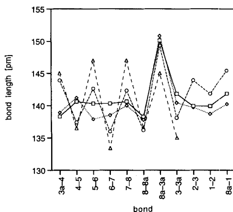
Fig. 4. Bond-length variation [pm] in 4-phenylbenz[ a ]azulene ( 4 ), 4-phenylazulene ( 5 ), azulene ( 6 ) [9], and heptafulvene ( 7 ) [10] (for numbering, see Footnote a in Table 1). ---○---: 4 ; .....◇.....: 5 ; —□—: 6 ; ---△---: 7 .
