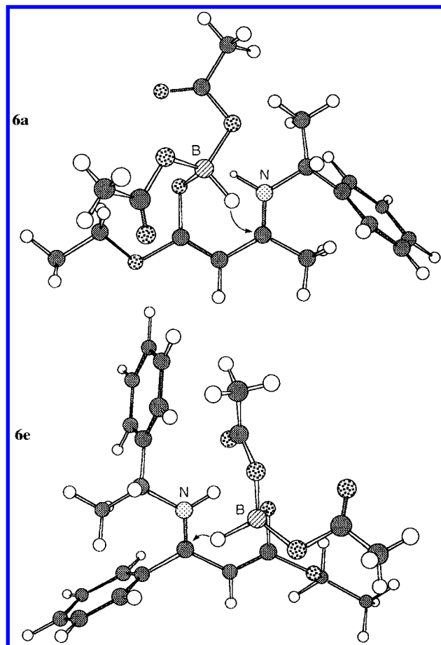
Figure 3. Hypotized, not minimized, transition-state model geometries for intramolecular hydride transfer in the case of enol ester–diacetoxyborohydride complexes 6a (top) and 6e (bottom, the rear view).
