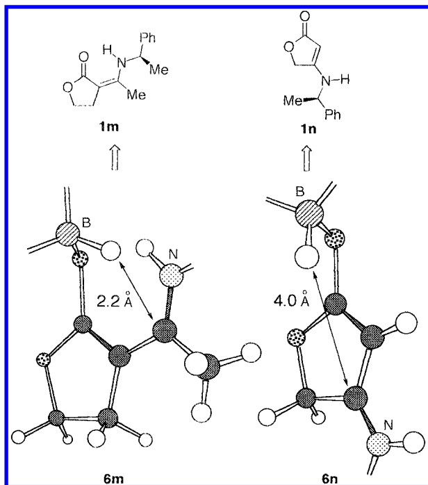
Figure 2. Comparative interaction of the BH and the electrophilic C=N groups in the s-cis ( 6m ) and the constrained s-trans ( 6n ) models of the intermediate enol ester–diacetoxyborohydride complexes. For clarity exemplified models were depicted.
