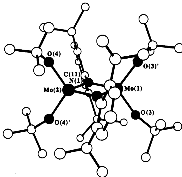
Figure 2. Drawing of the structure of [Mo(NAr)(O- t -Bu) 2 ] 2 (12).
