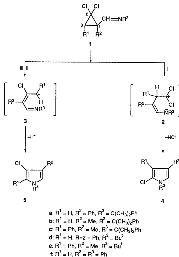
Scheme 1 Reagents and conditions: i, 1,3-bond fission; ii, Cl − ; iii, 3-bond fission
