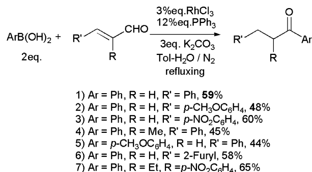
Scheme 2 Rh-catalysed self-conjugate reduction, cross-coupling tandem reaction of cinnamaldehydes with arylboronic acids.
