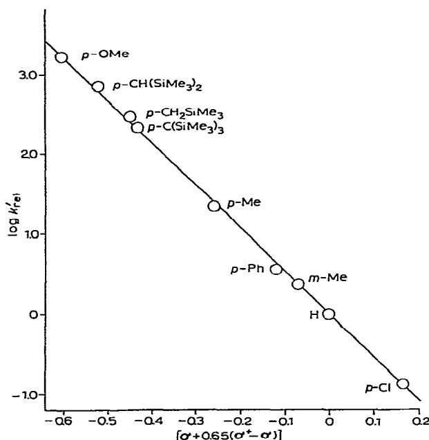
Fig. 1. Plot of \log k'_{\text{rel}} against [\sigma + 0.65(\sigma^+ - \sigma)] for cleavage of \text{XC}_6\text{H}_4\text{SiMe}_3 compounds by aqueous methanolic perchloric acid.
